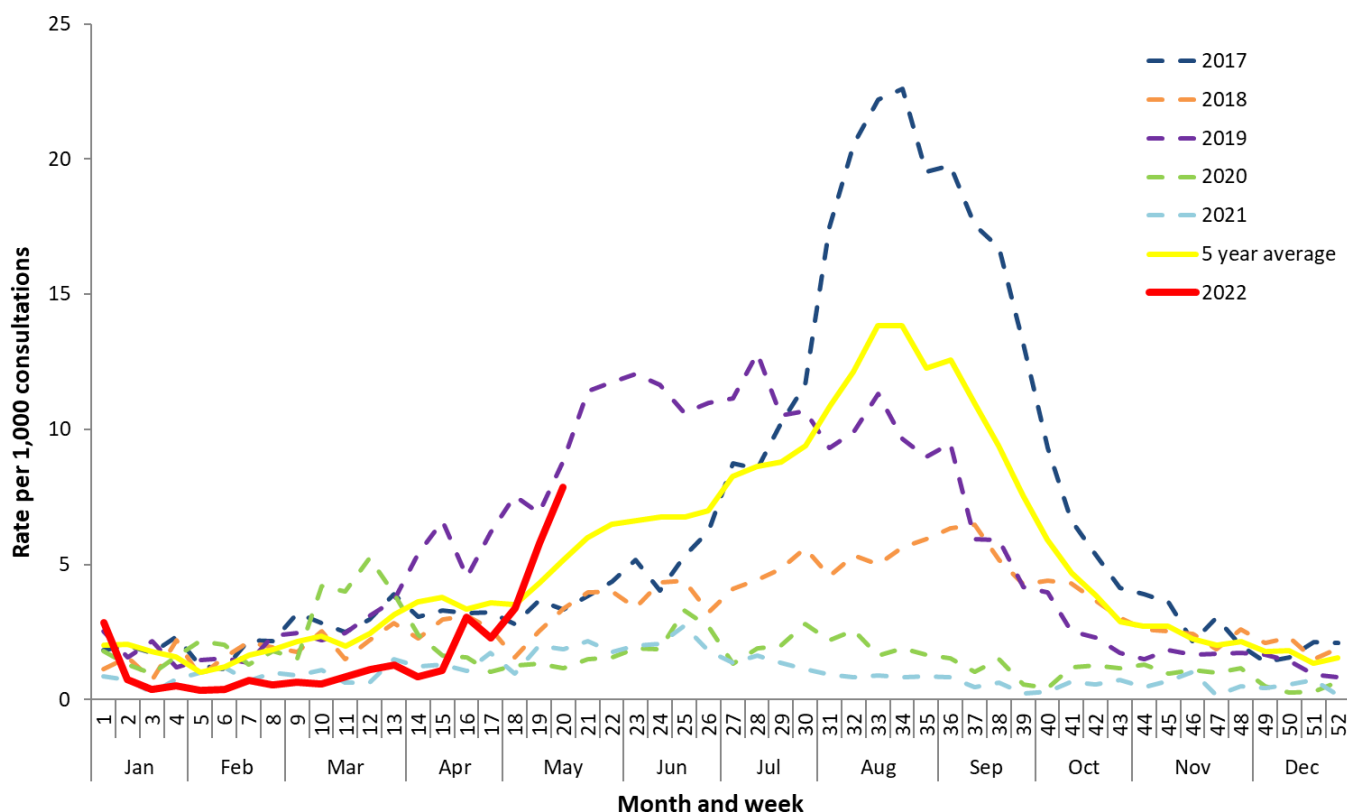
Figure 3. Unweighted rate of ILI reported from ASPREN sentinel GP surveillance systems, Australia, 01 January 2017 to 22 May 2022, by month and week**
