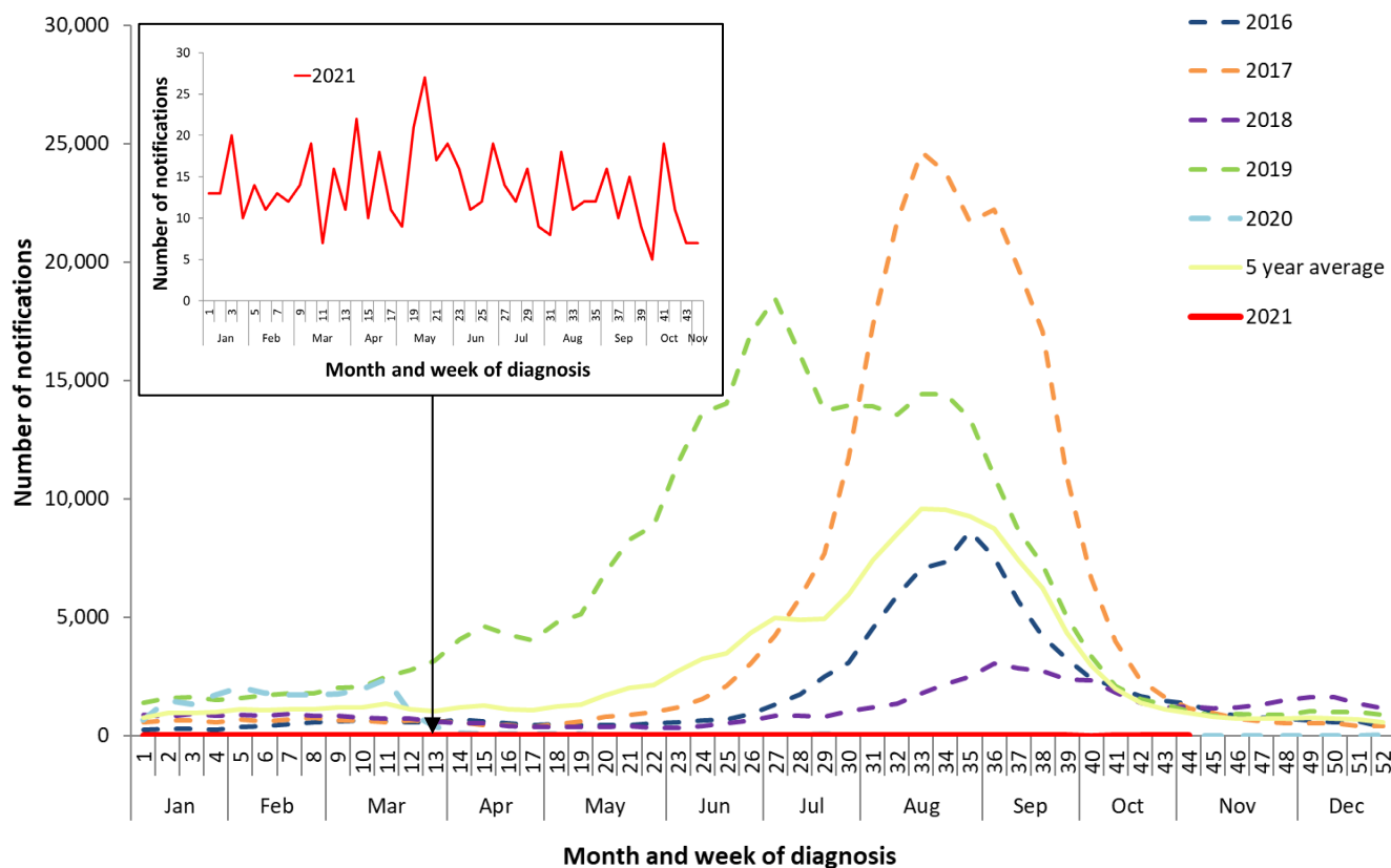
Figure 4. Notifications of laboratory-confirmed influenza, Australia, 01 January 2016 to 07 November 2021, by month and week of diagnosis*
