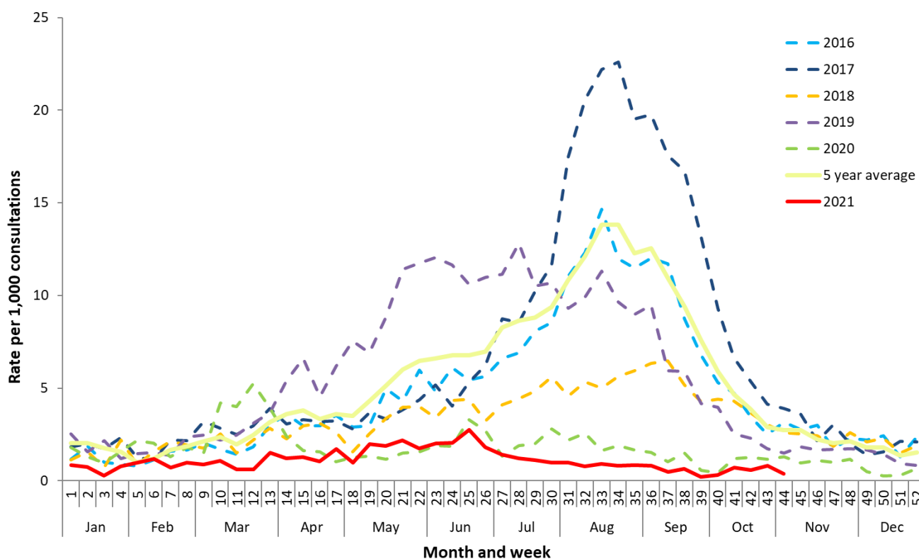
Figure 3. Unweighted rate of ILI reported from ASPREN sentinel GP surveillance systems, Australia, 01 January 2016 to 07 November 2021, by month and week**
