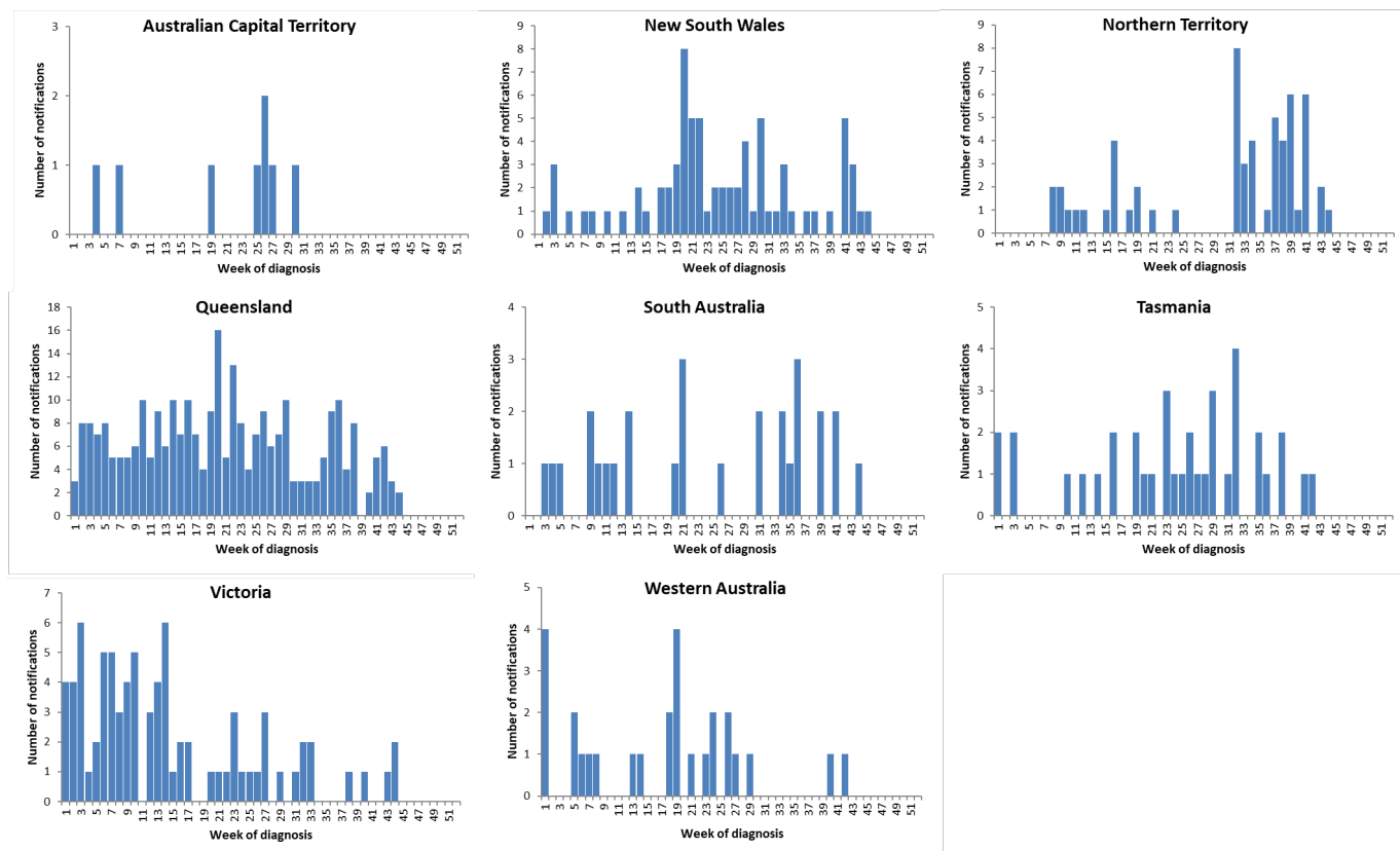
Figure 5. Notifications of laboratory-confirmed influenza*, 01 January to 07 November 2021, by state or territory and week of diagnosis
