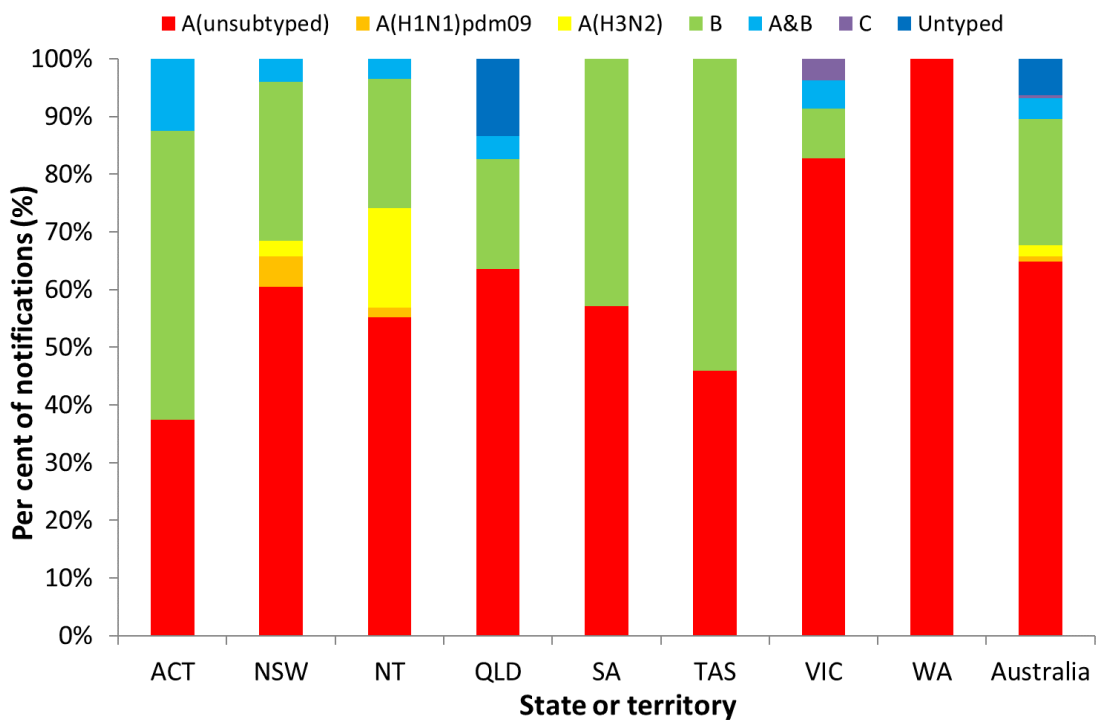
Figure 8. Per cent of notifications of laboratory-confirmed influenza, Australia, 01 January to 07 November 2021, by subtype and state or territory*
