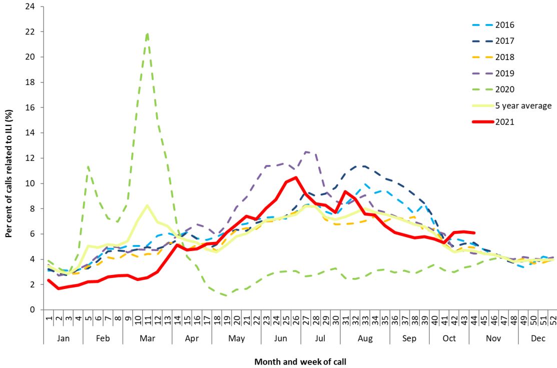
Figure 1. Per cent of calls to Healthdirect related to ILI, Australia, 01 January 2016 to 07 November 2021, by month and week of call*
