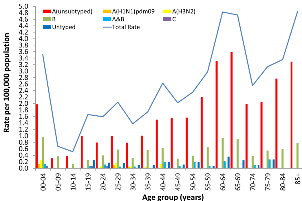
Figure 6. Rate of notifications of laboratory-confirmed influenza, Australia, 01 January to 07 November 2021, by age group and subtype
