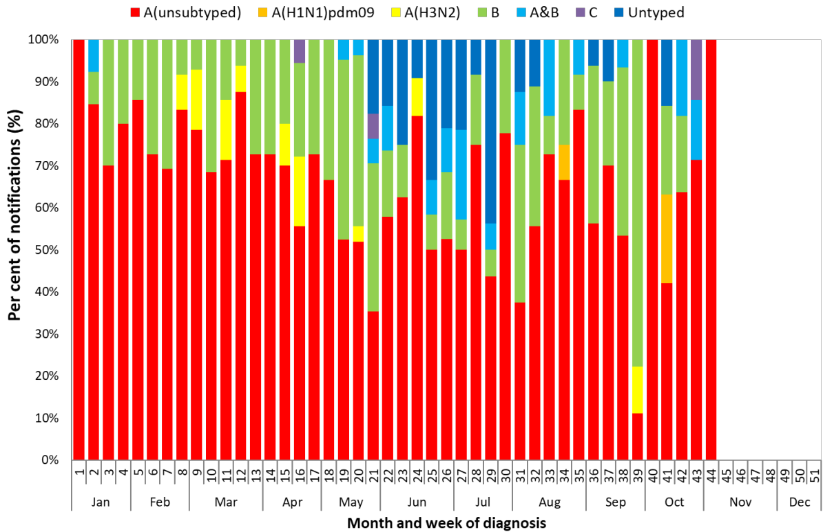
Figure 7. Per cent of laboratory-confirmed influenza, Australia, 01 January to 07 November 2021, by subtype and week of diagnosis*
