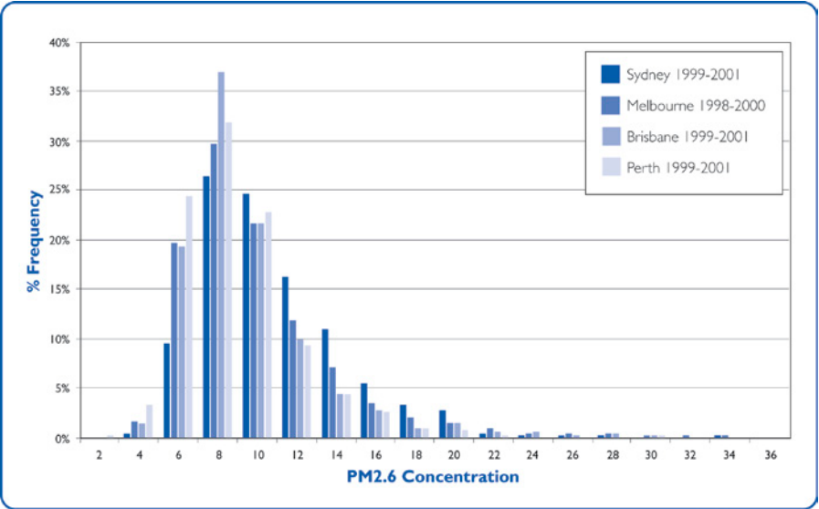
Figure 5.6.1b: Frequency distribution of composite daily 24-hour PM 2.5
