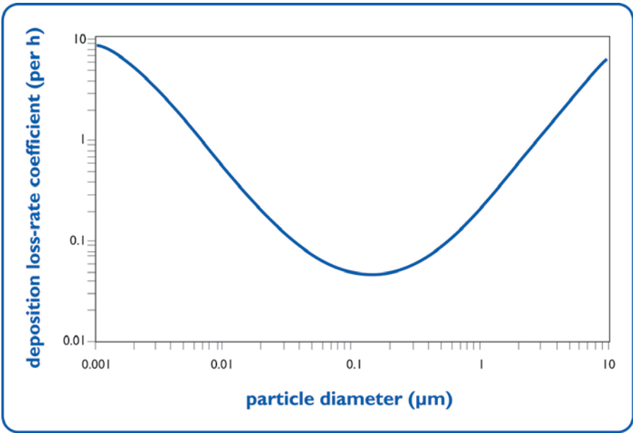
Figure 5.3.1: Particle size/diameter versus deposition rate
