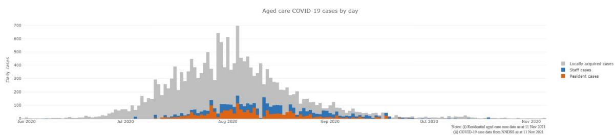
Figure 2: Number of daily reported COVID-19 cases in Australian residential aged care Facilities overlayed with national locally acquired cases 5 .
