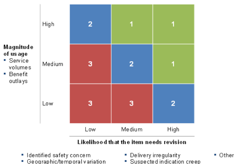
Figure 1: Prioritisation matrix
