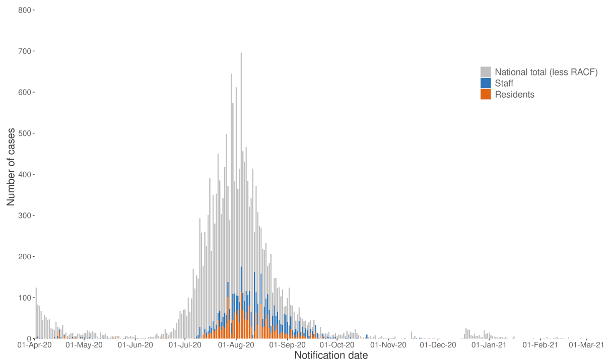
Figure 2: Number of daily reported COVID-19 cases in Australian residential aged care facilities overlaid with national locally acquired cases 4 .
