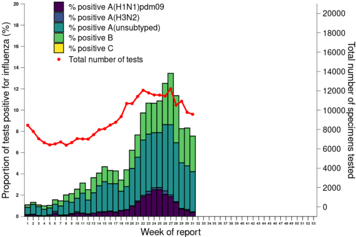
Figure 4: Proportion of sentinel laboratory tests positive for influenza and total number of specimens tested, 1 January to 6 August 2023, by subtype, year and week*
